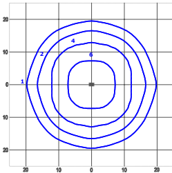
lux UCRA95SHA40K Mounting Height: 6m
